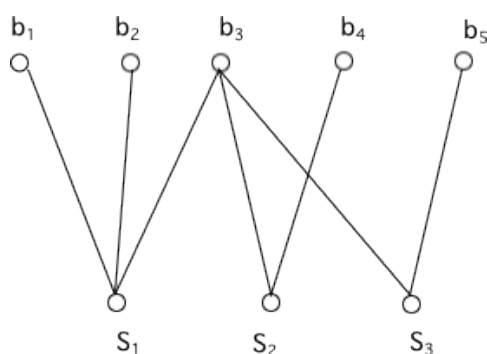
Example of a buyer-seller network
