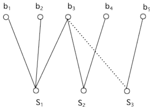
Removal of a link
